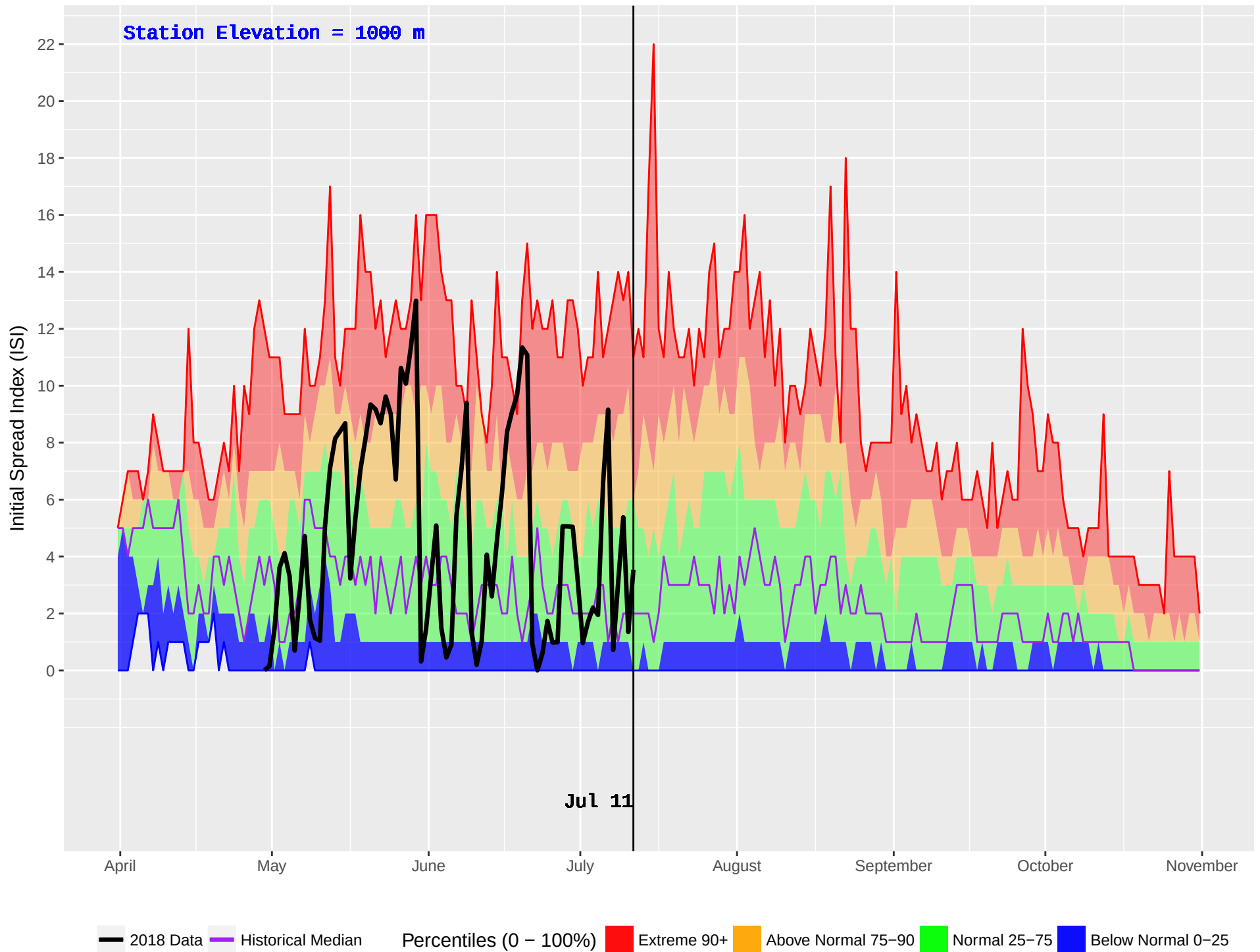
SUCCOUR CREEK (374) : Historical (1986–2016) and Current (2018) Noon Initial Spread Index (ISI)
