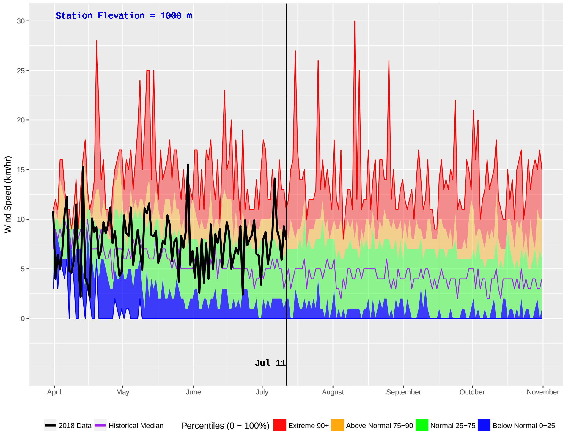
SUCCOUR CREEK (374) : Historical (1986–2016) and Current (2018) Noon Wind Speed
