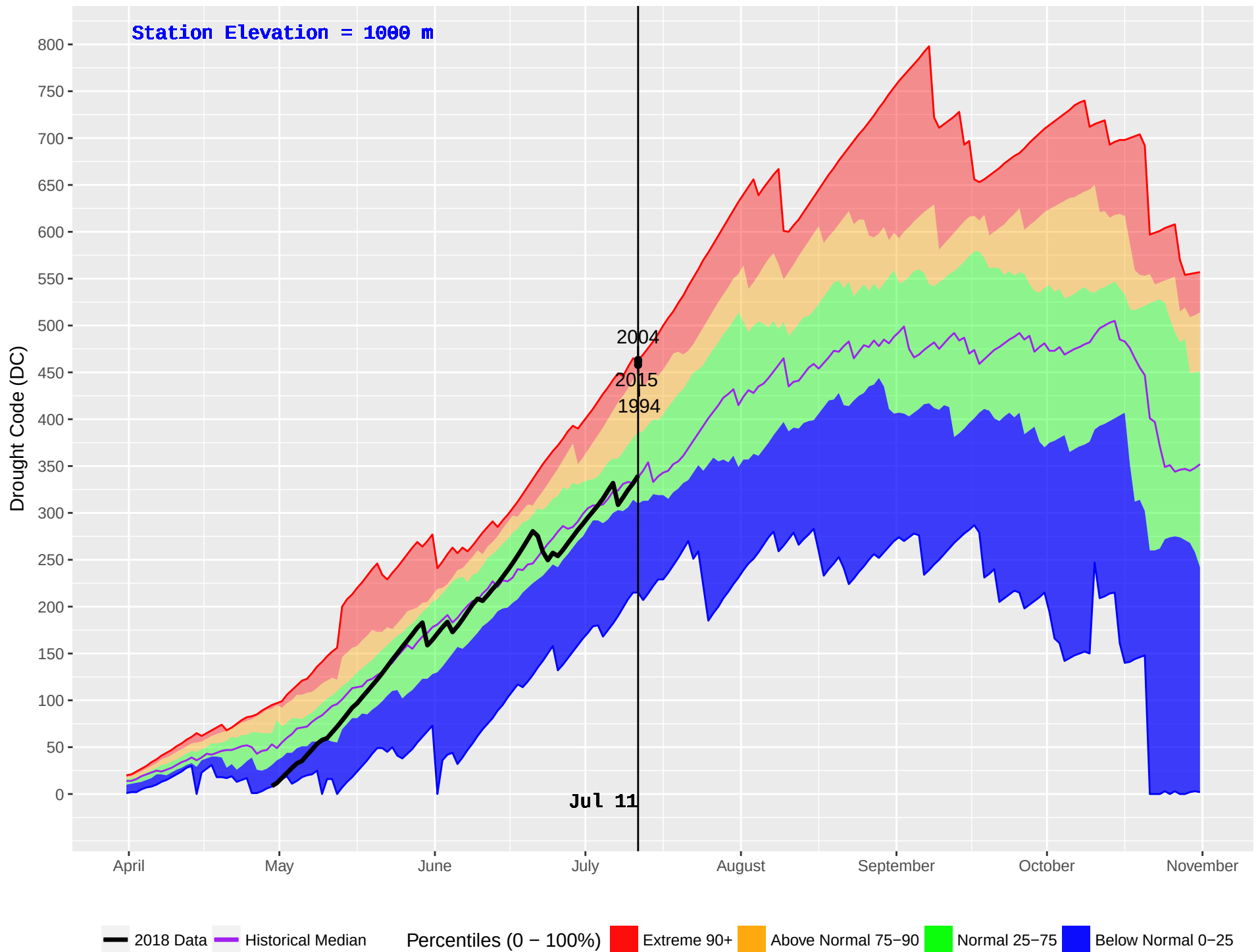
SUCCOUR CREEK (374) : Historical (1986–2016) and Current (2018) Noon Drought Code (DC)
