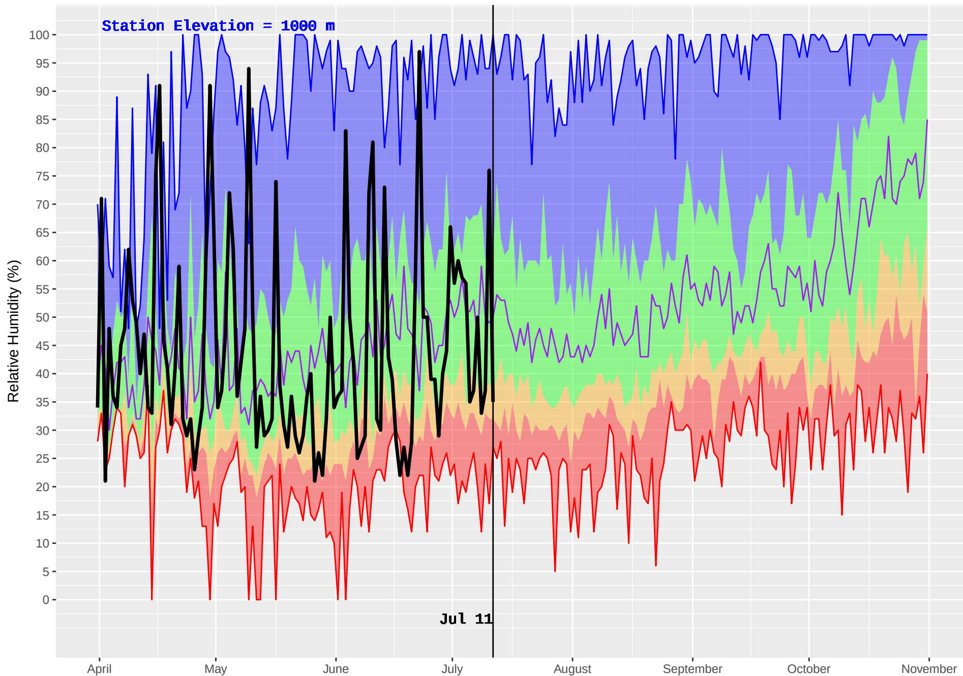
SUCCOUR CREEK (374) : Historical (1986–2016) and Current (2018) Noon Relative Humidity
