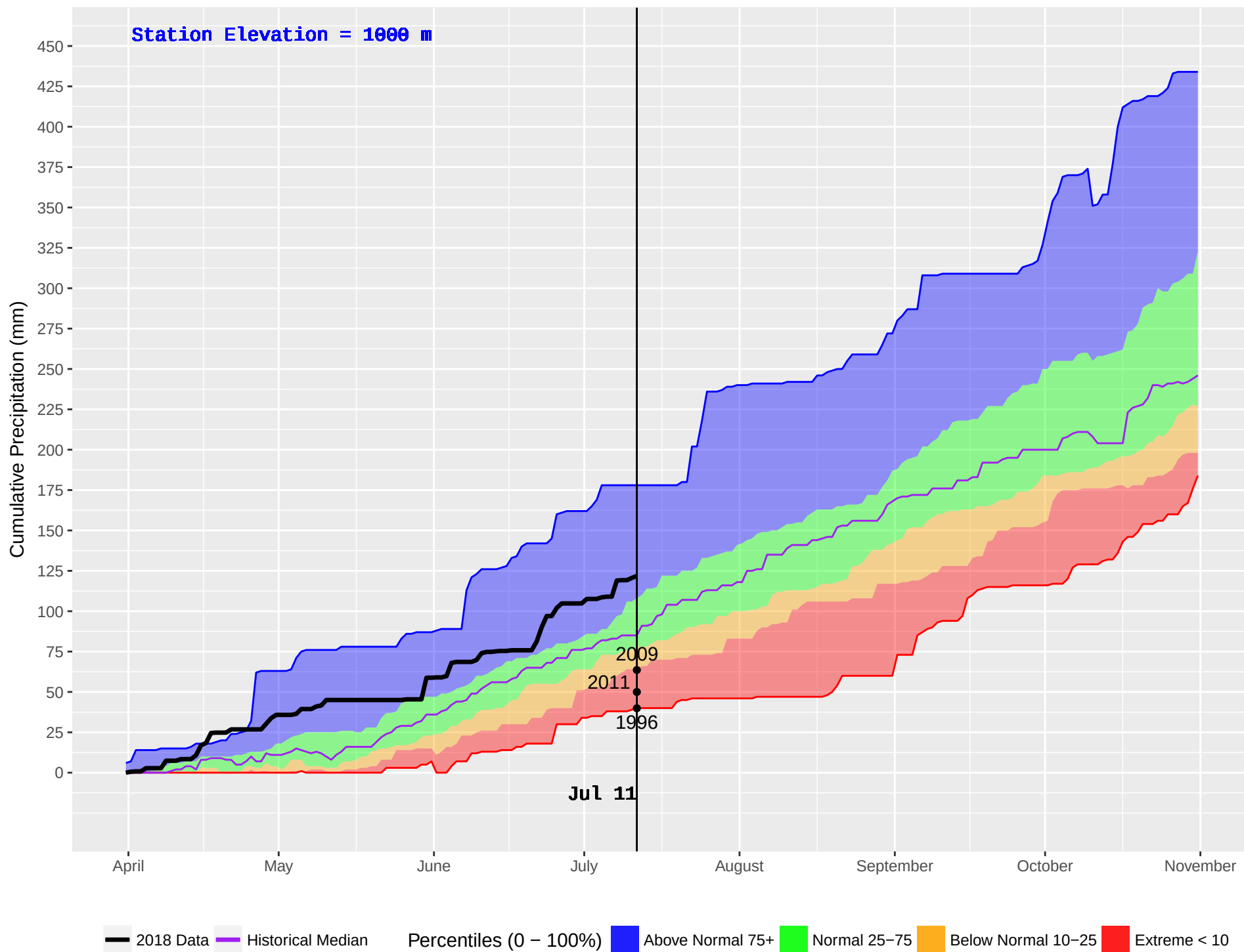
SUCCOUR CREEK (374) : Historical (1986–2016) and Current (2018) Noon Cumulative Precipitation
